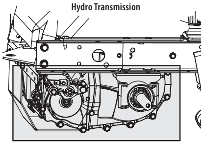
Wheel Not Shown for Clarity
