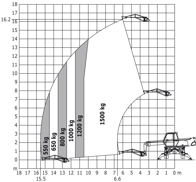
Rotation on lowered stabilisers with 1500 kg jib Metric
