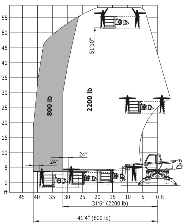
Rotation on lowered stabilisers with 365/1000 kg platform Imperial
