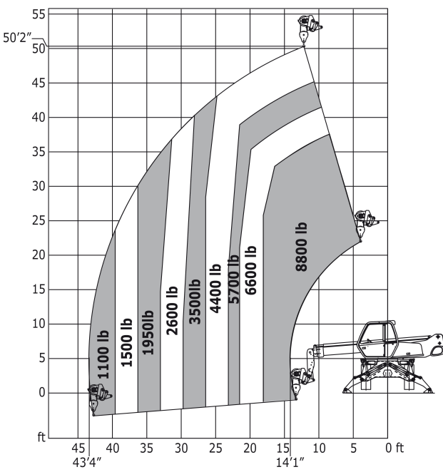
Rotation on lowered stabilisers with winch 5000 kg Imperial
