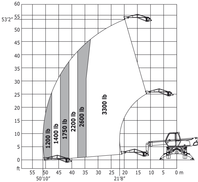
Rotation on lowered stabilisers with 1500 kg jib Imperial
