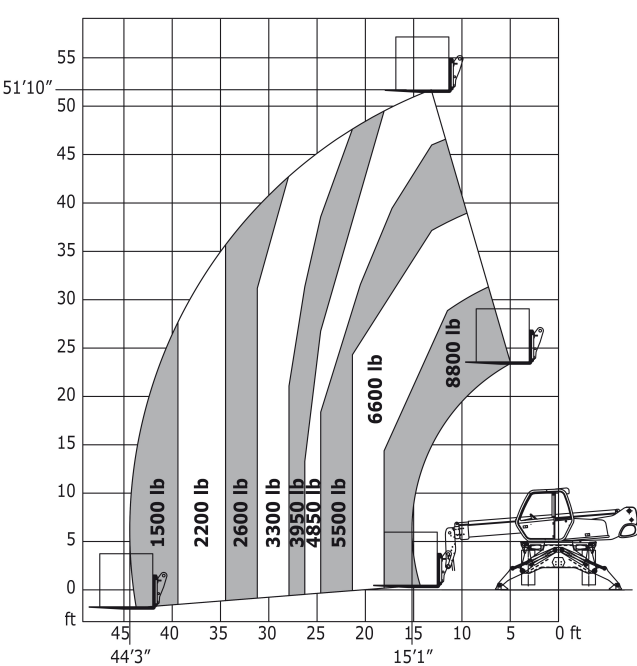
Rotation on lowered stabilisers with forks Imperial
