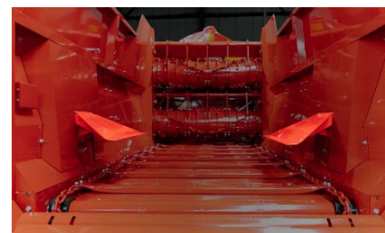
Hydraulic Bale Lift Plates SC4902
