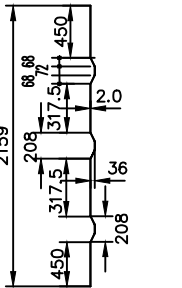
SECTION G-G
