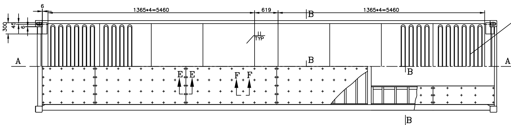
SECTION G-G
