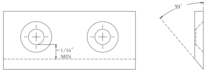
Figure 13- Chipper knife minimum cutting edge
