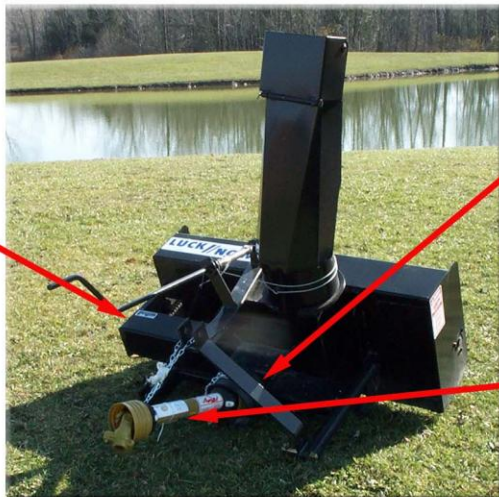
Shear bolt protection
