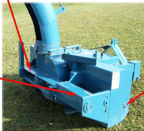
Shear bolt protection
