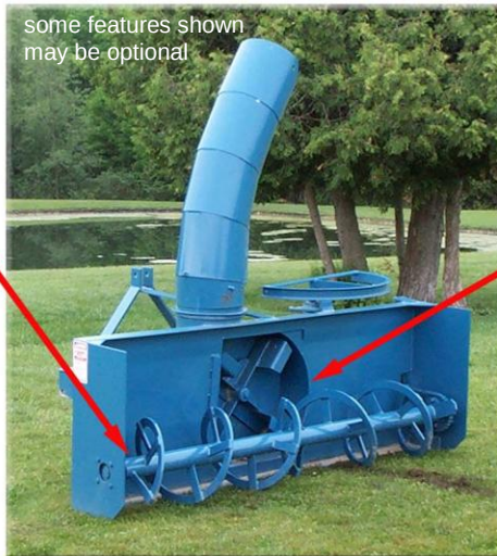
Heavy augers and shafts
