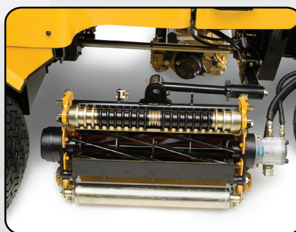
Rear cutting units rotate out and up for easy maintenance
