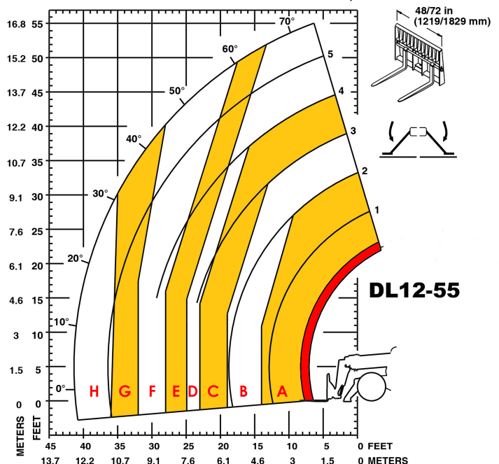
Machine on stabilizers with forks Imperial
