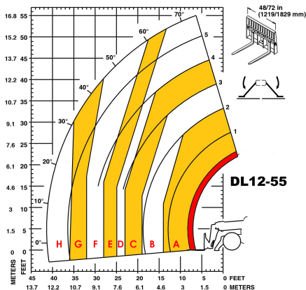
Load Chart Other Imperial
