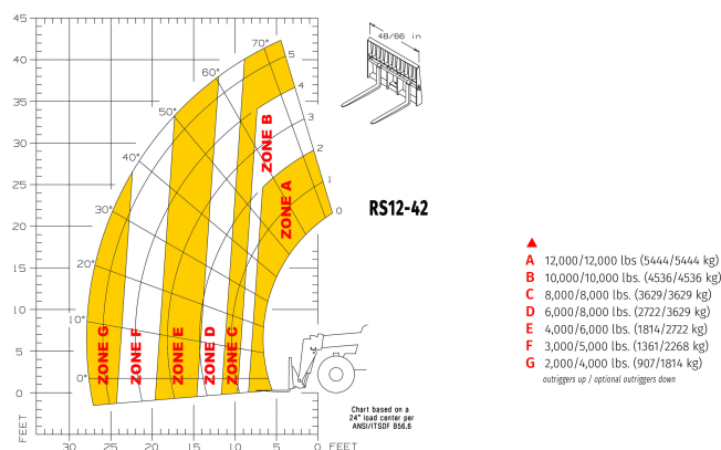
Load Chart imperial
