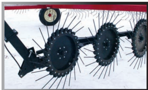
2 or 3 wheel center kicker assembly available.
