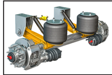
Disc Brakes
