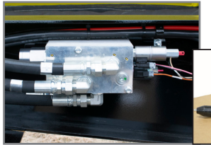
EOH Valve and Control Box
