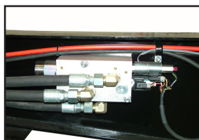
Trailer Mounted Electric Over Hydraulic Control Valve
