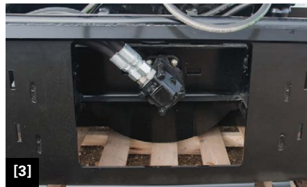
[1] Hydraulic motor chain drive. [2] Wiring harness fits most skid steer brands. [3] A hydraulic motor mounts directly on the fan and auger shaft eliminating couplers and chain drive assembly.
