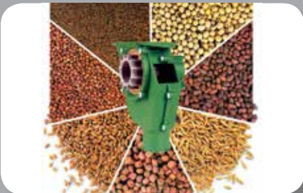
FLUTED FEED CUP - Provides gentle and even delivery of a wide variety of seed sizes and shapes.
