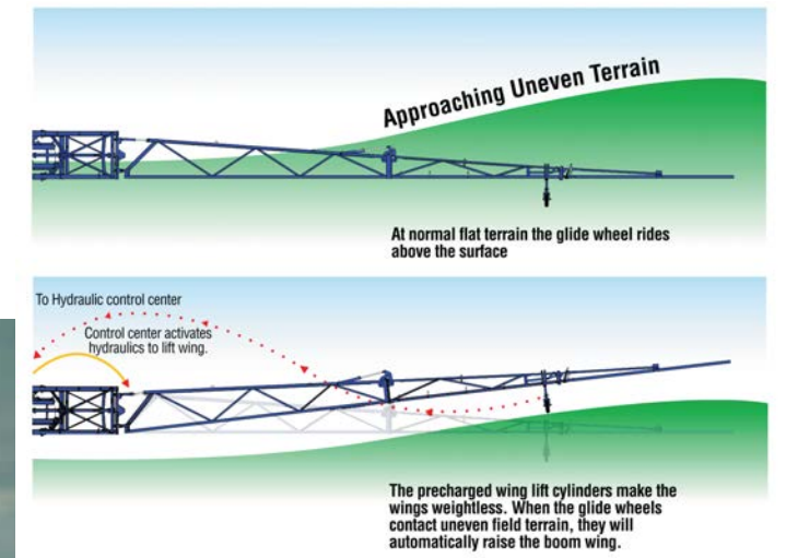
Cab mounted console allows operator to adjust the precharge on the wing lift cylinders for optimal boom performance.
