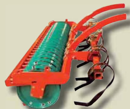
Levelling tines
