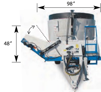
Options: Flip-up Conveyor (Right Side)
