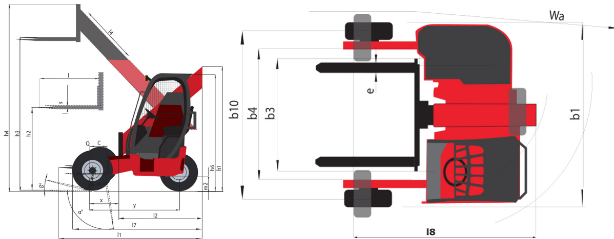
TMT 55 HT 4W - Dimensional drawing
