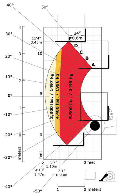
Machine on stabilizers with forks Metric
