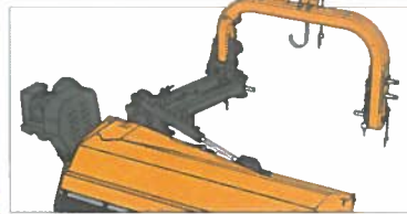
FERRI PATENT on DOUBLE LINKAGE This system utilizes a three point headstock attachment with a double linkage. One machine is able to perform the work which required use of two slope mowers.
