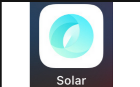
User Friendly
