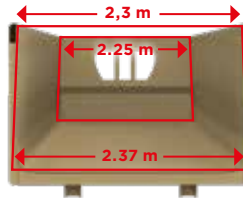
Tapered body (2.25 m at the front and 2.3 m at the rear), wider at the bottom than at the top to facilitate unloading.
