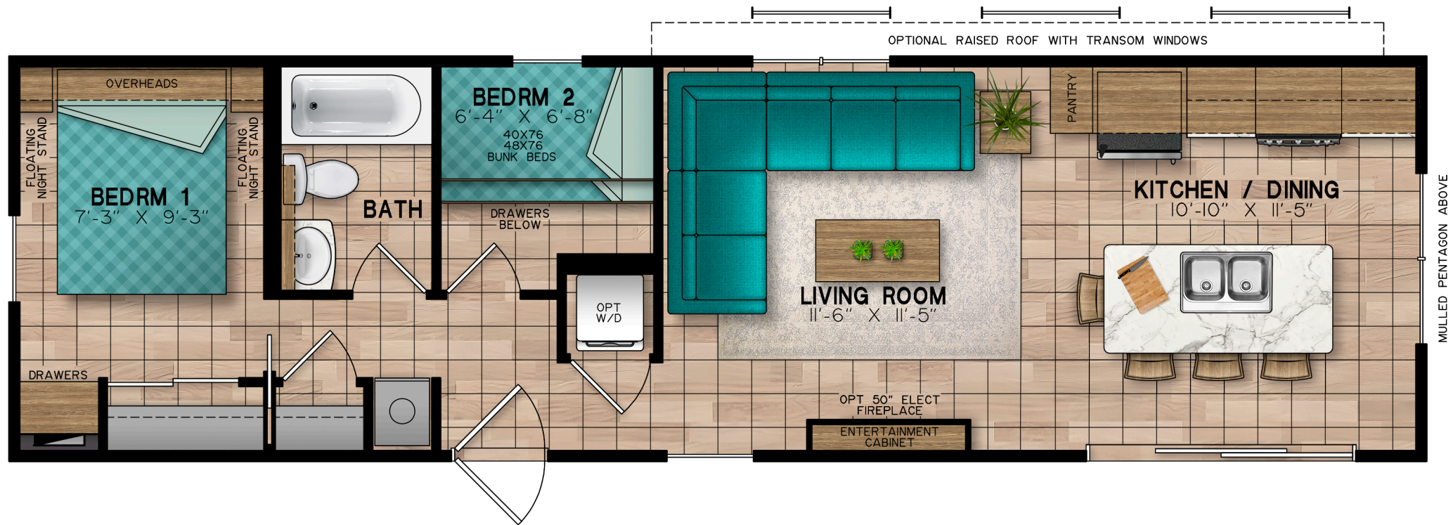
Ajax 23-4998-2 42' x 12' All Season (504sq.ft.)
