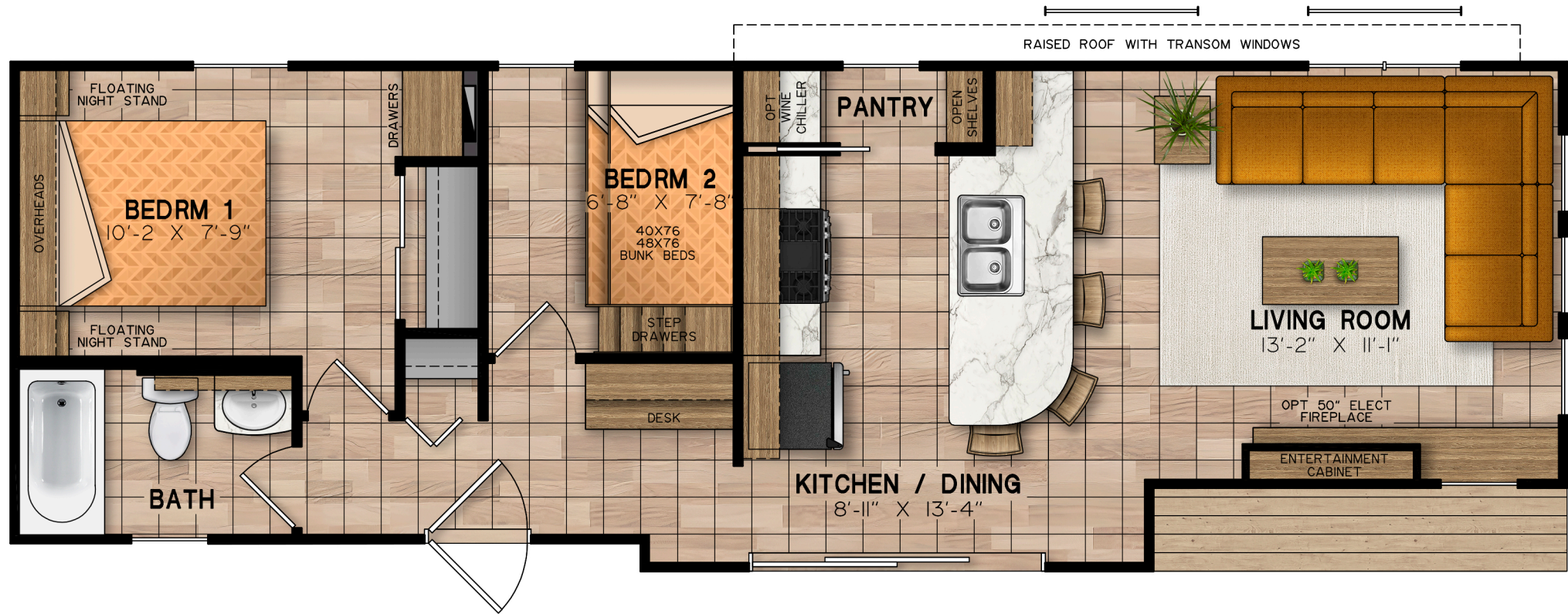
Erie 23-4963-2TR 42' x 13' Escape (540sq.ft)
