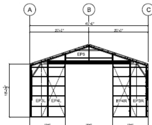
2 WEST END PANEL LAYOUT
