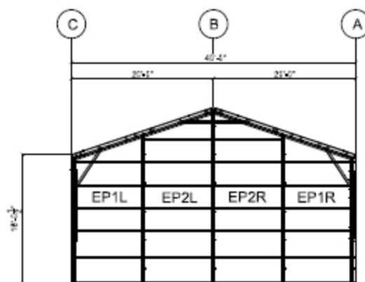
3 EAST END PANEL LAYOUT
