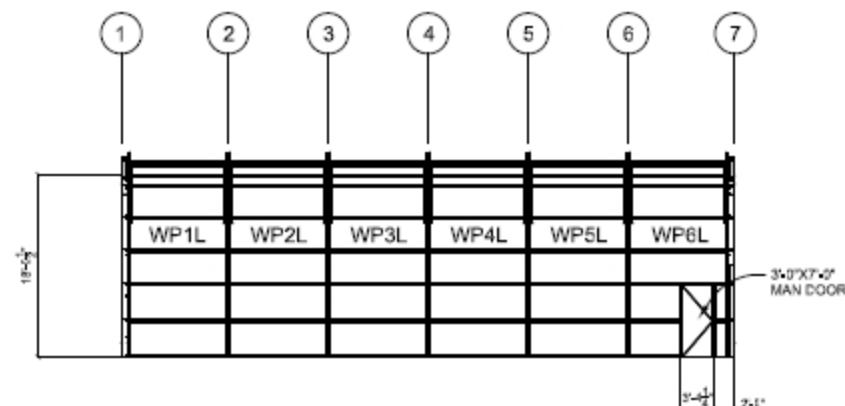
4 SOUTH WALL PANEL LAYOUT
