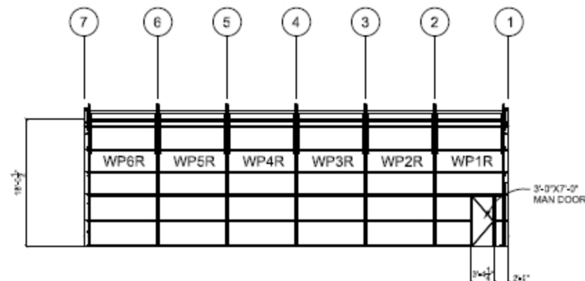
5 NORTH WALL PANEL LAYOUT
